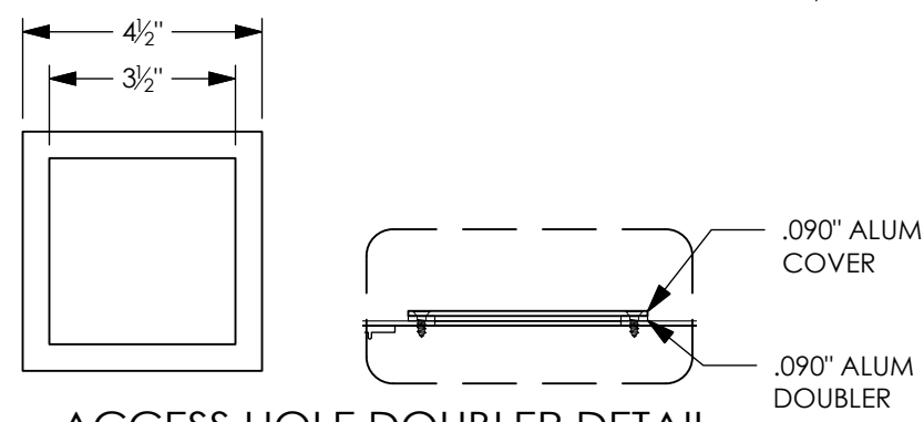
ACCESS HOLE DOUBLER DETAIL SCALE: 1/4" = 1"
