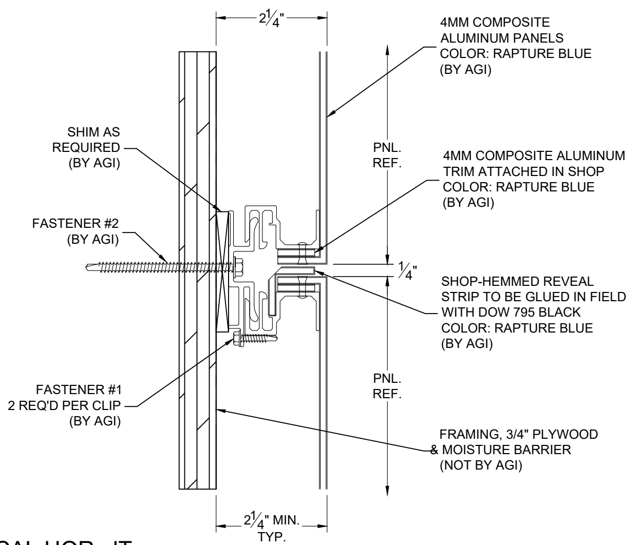
2 TYPICAL HOR. JT. D01 6"=1'-0"
