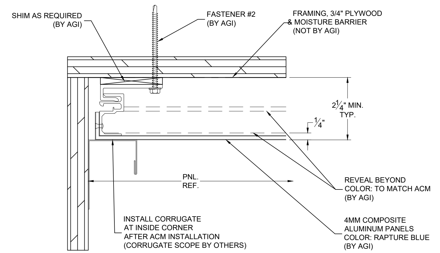
3 LEFT TERMINATION DETAIL D01 6"=1'-0"
