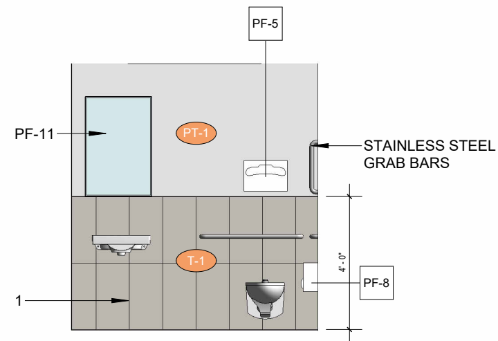
2 | RECEPTION RESTROOM 1/4" = 1'-0"
