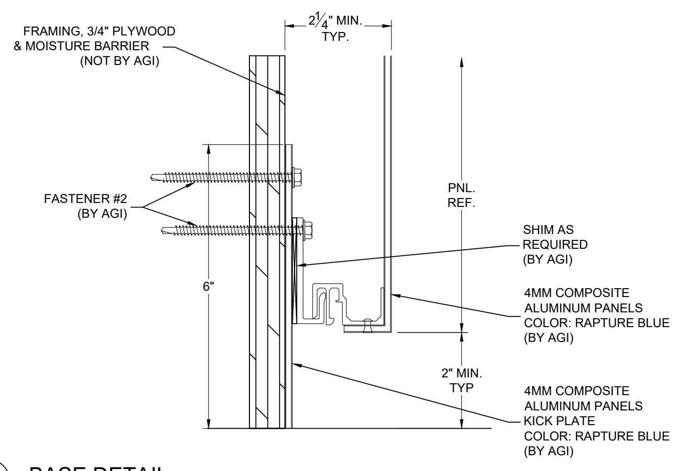
4 BASE DETAIL D01 6"=1'-0"
