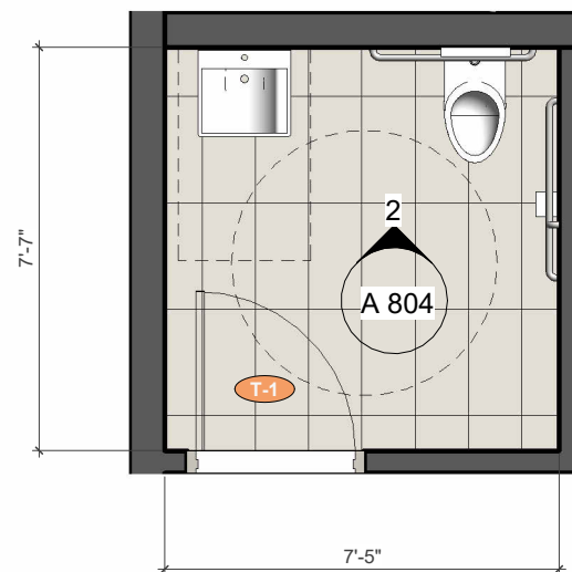
1 | FIRST FLOOR TOILET ROOM 1/4" = 1'-0"
