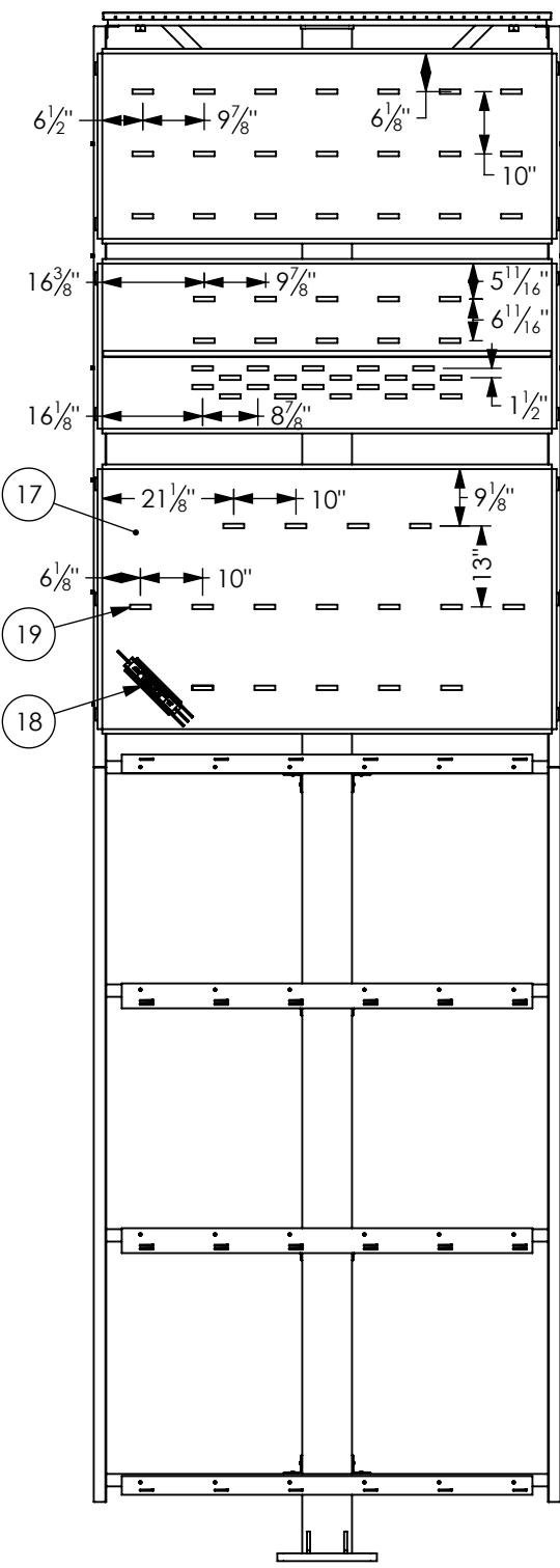
ELECTRICAL ELEVATION
