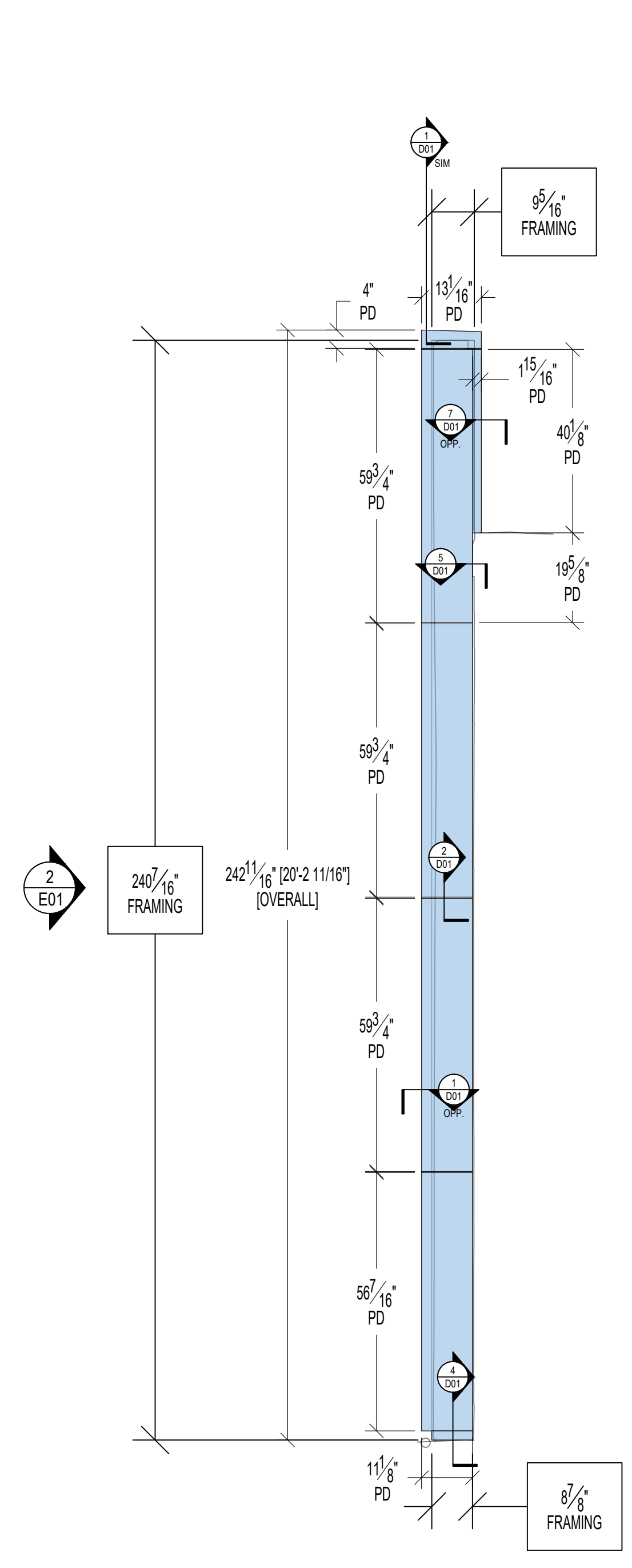
3 FORD PRO RIGHT ELEVATION E01 1/2"=1'-0"
