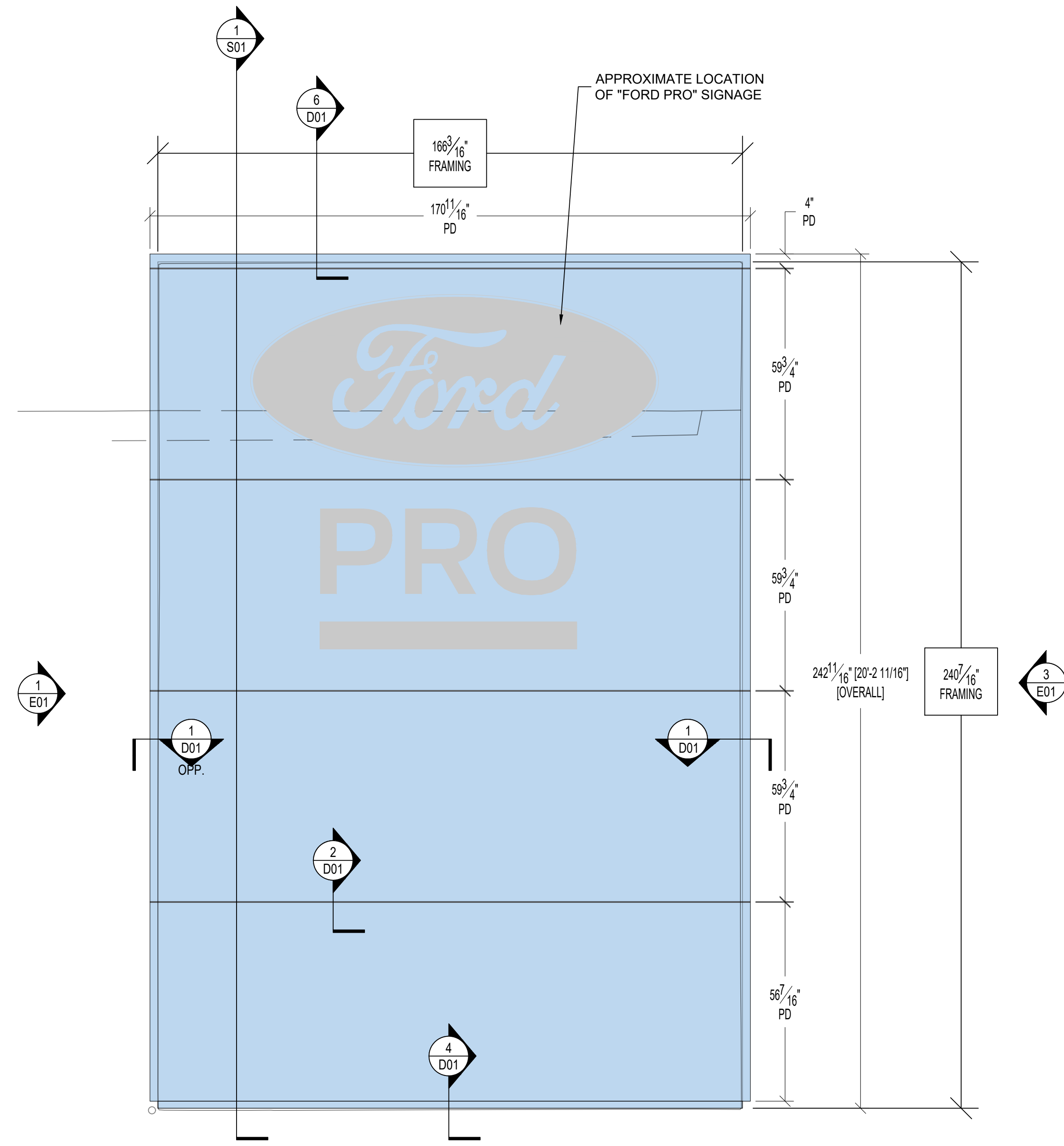
2 FORD PRO FRONT ELEVATION E01 1/2"=1'-0"
