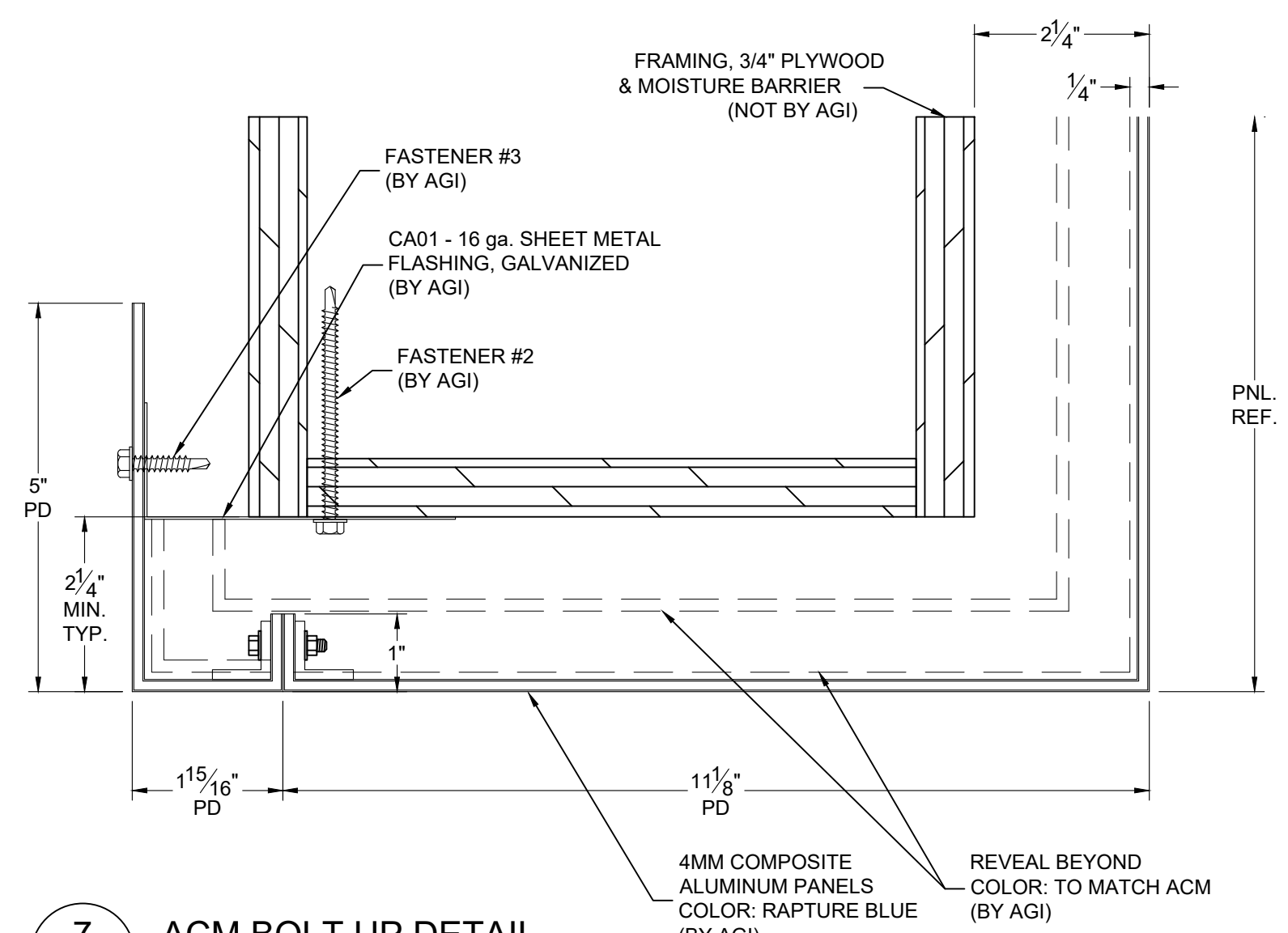
7 ACM BOLT UP DETAIL D01 6"=1'-0"
