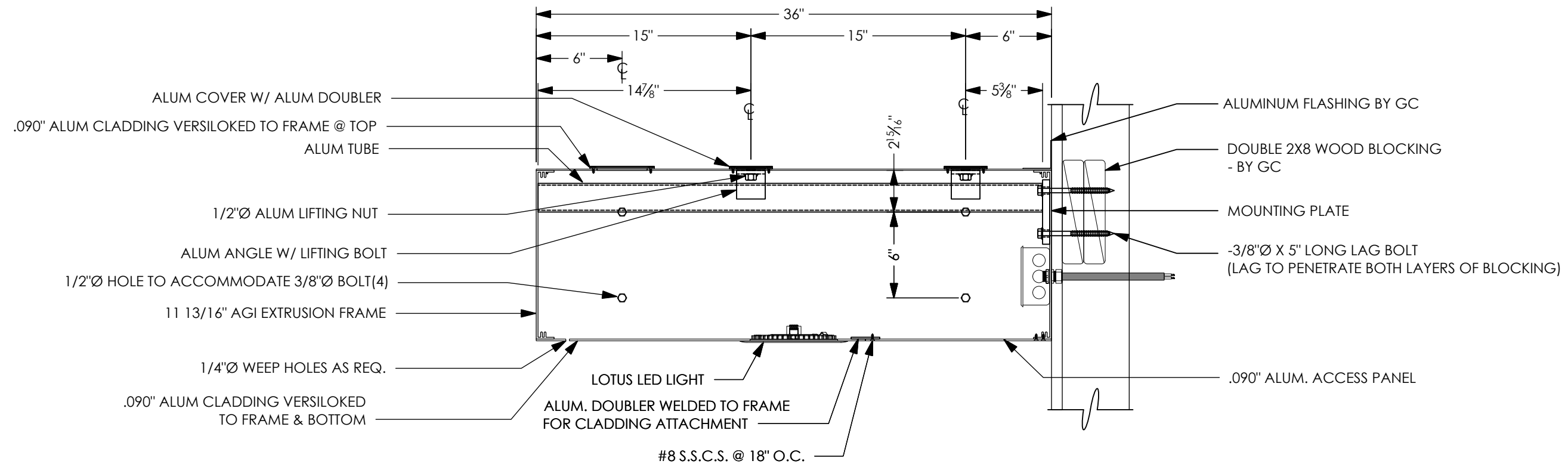
SIDE SECTION VIEW WOOD BLOCKING MOUNTING SCALE: 1/8" = 1"
