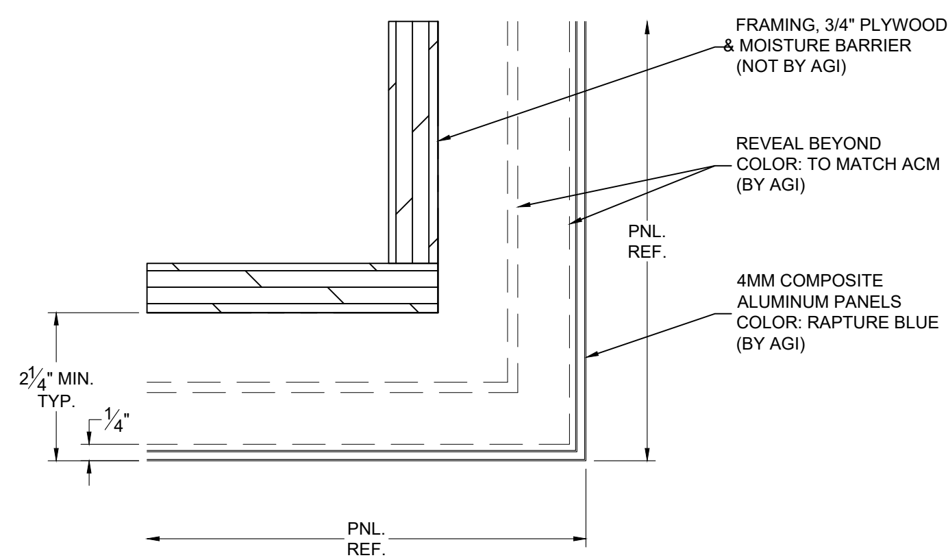
1 OUTSIDE CORNER DETAIL D01 6"=1'-0"
