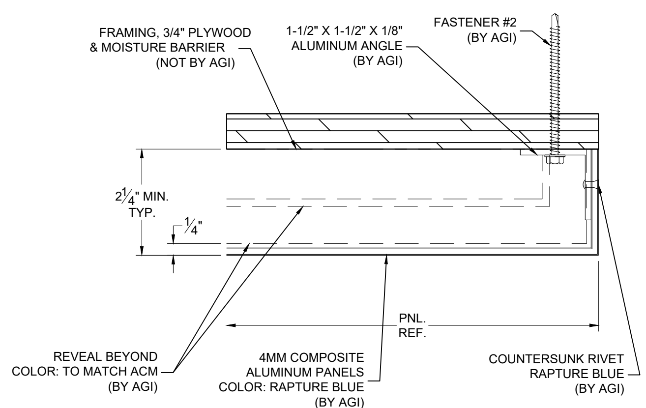
5 RIGHT TERMINATION DETAIL D01 6"=1'-0"
