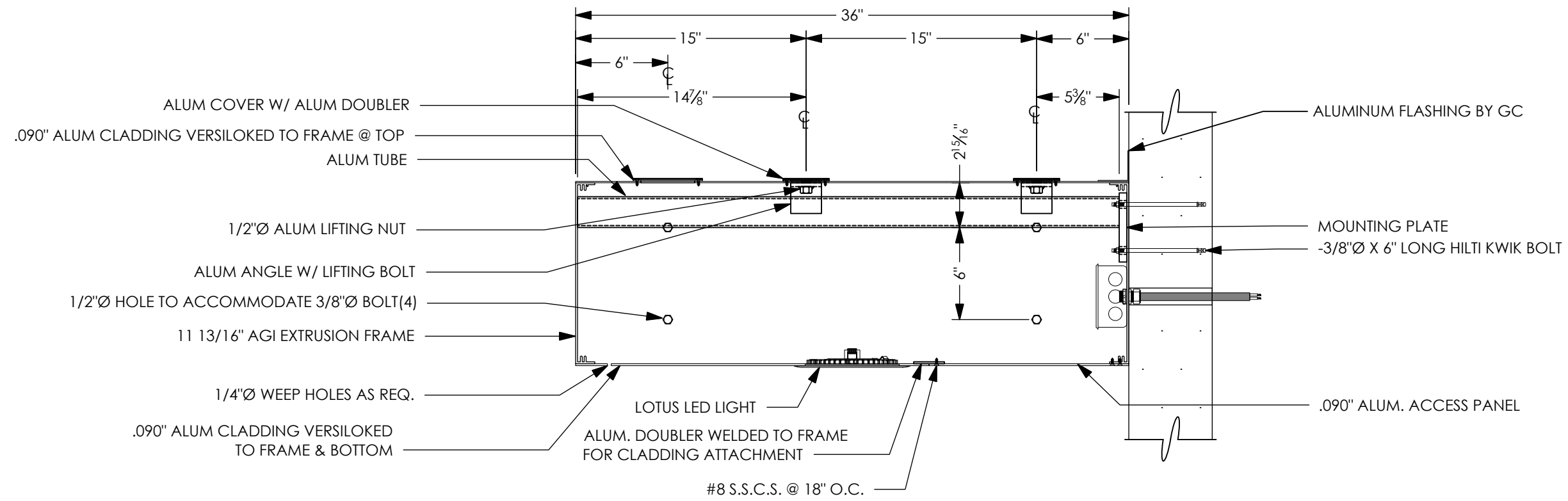
SIDE SECTION VIEW CONCRETE MOUNTING SCALE: 1/8" = 1"
