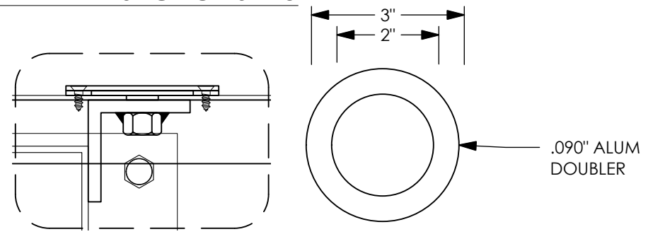
LIFTING HOLE DOUBLER DETAIL SCALE: 3/8" = 1"
