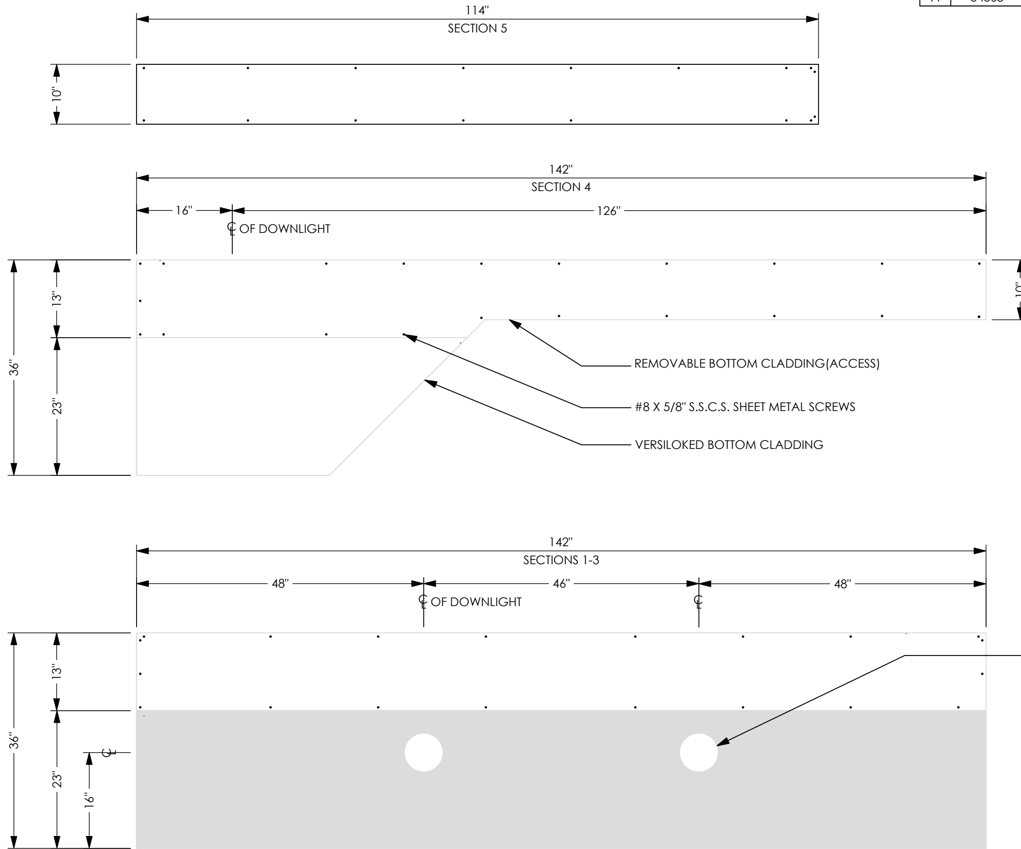
REMOVABLE CLADDING PLAN VIEW SCALE: 3/4" = 1'-0"
