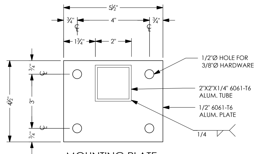
MOUNTING PLATE SCALE: 3/8" = 1"
