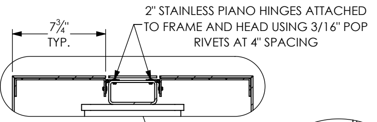
DETAIL F SCALE 1 : 8
