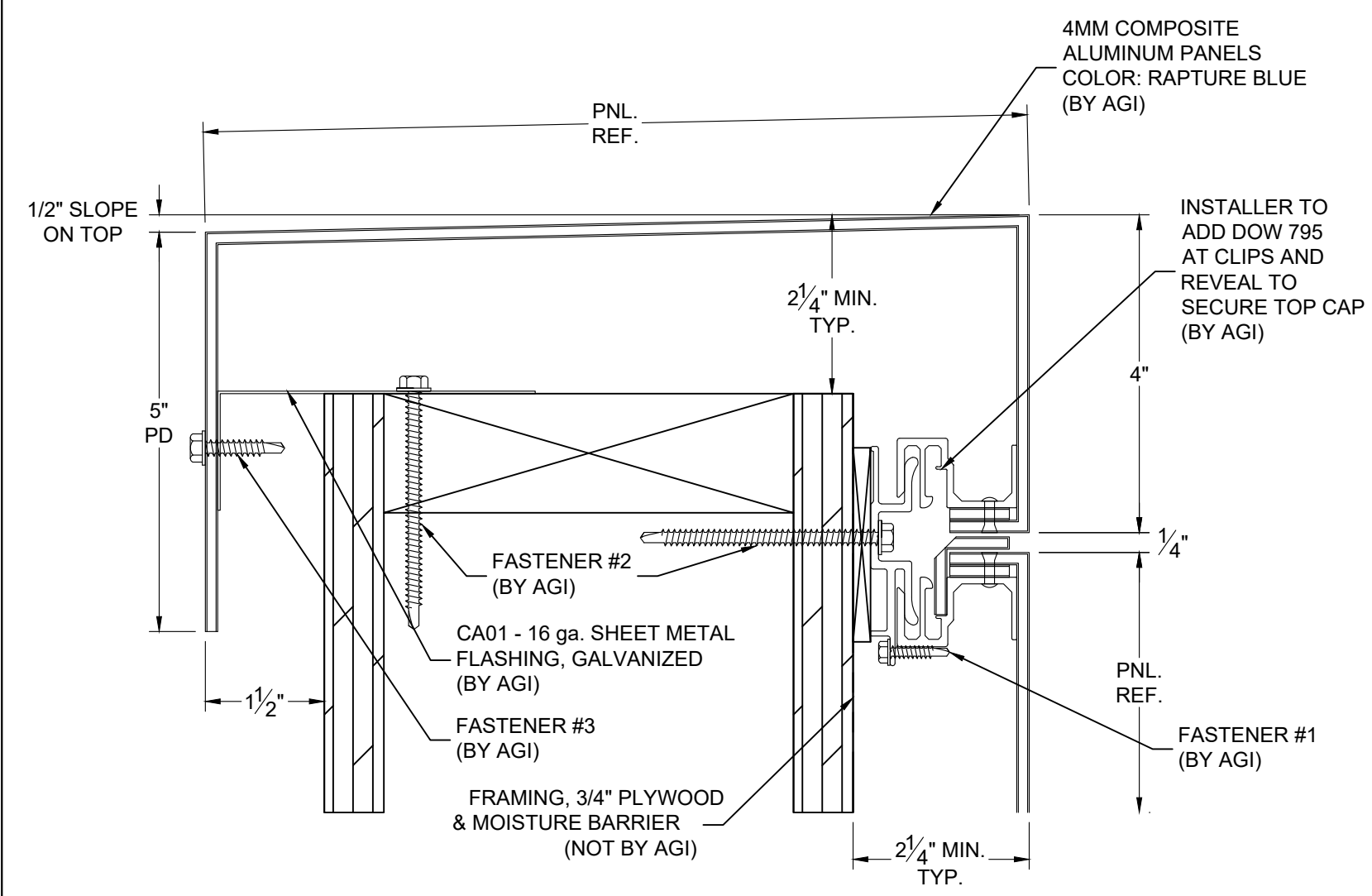
6 ACM COPING DETAIL D01 6"=1'-0"
