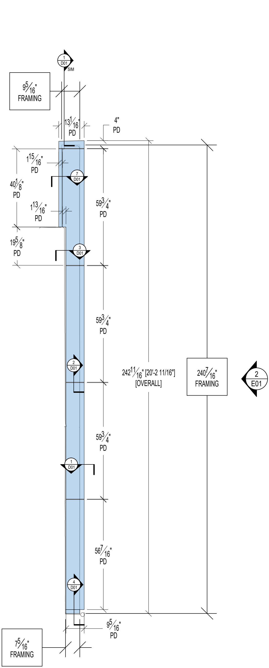
1 FORD PRO LEFT ELEVATION E01 1/2"=1'-0"
