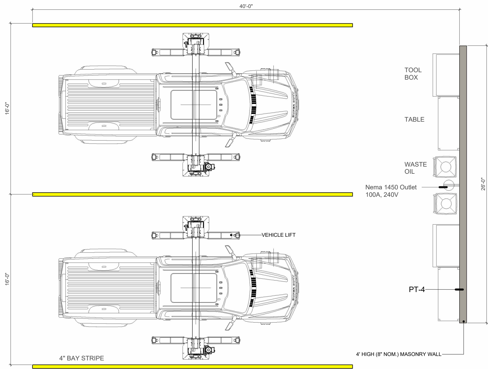
1 | TYP. SERVICE BAY/ EQUIPMENT 3/16" = 1'-0"
