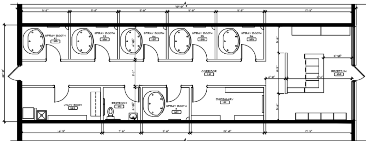
1 PRELIMINARY FLOOR PLAN - 1,400 SF LEASE SPACE SCALE: 1/4" = 1'-0"
